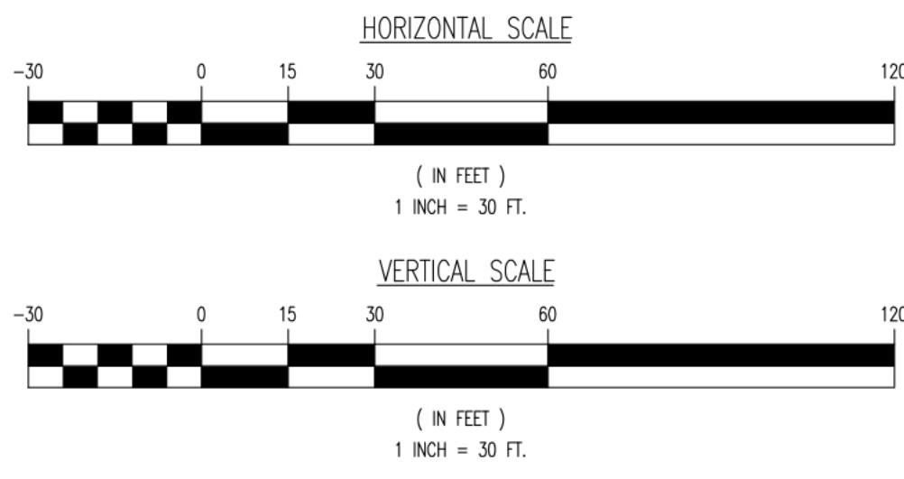
PROFILE VIEW OF SITE PROFILE 2 HORIZONTAL SCALE: 1"=30' VERTICAL SCALE: 1"=30'
