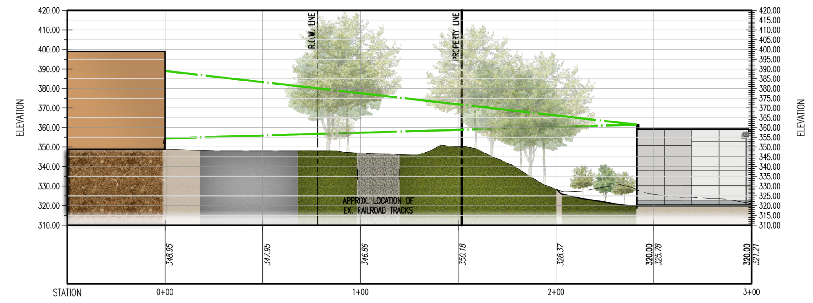
PROFILE VIEW OF SITE PROFILE 2 HORIZONTAL SCALE: 1"=30' VERTICAL SCALE: 1"=30'
