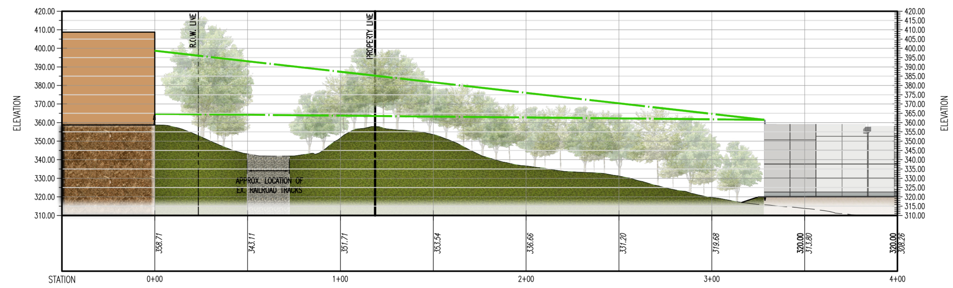
PROFILE VIEW OF SITE PROFILE 1 HORIZONTAL SCALE: 1"=30' VERTICAL SCALE: 1"=30'
