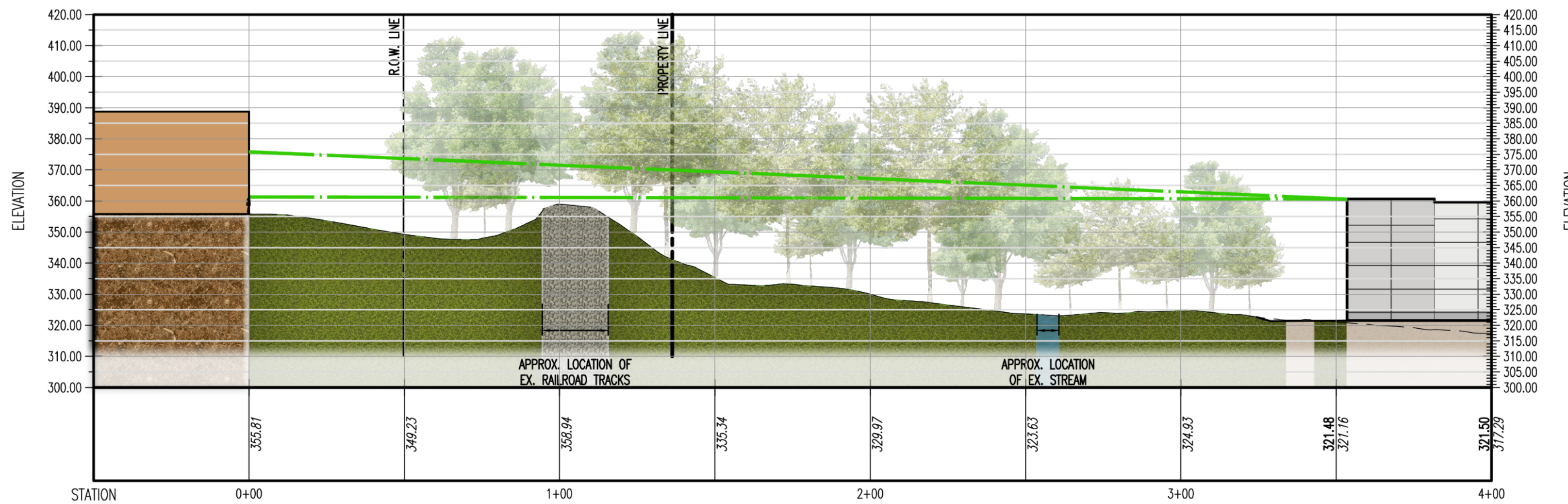
PROFILE VIEW OF SITE PROFILE 3 HORIZONTAL SCALE: 1"=30' VERTICAL SCALE: 1"=30'
